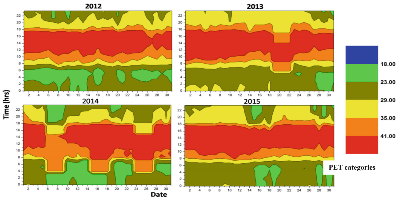
Fig. 4 PET (°C) over Anantapur District of Andhra Pradesh during May
