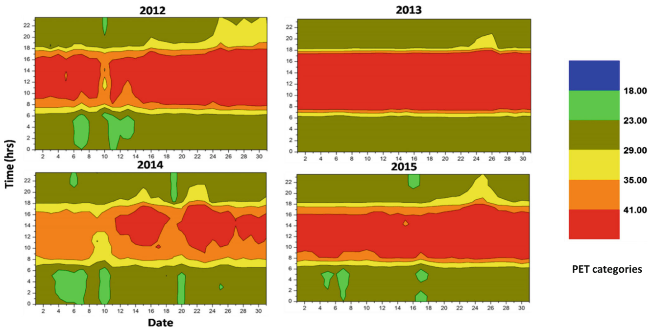
Fig. 7 PET (°C) over Undi District of Andhra Pradesh during May
