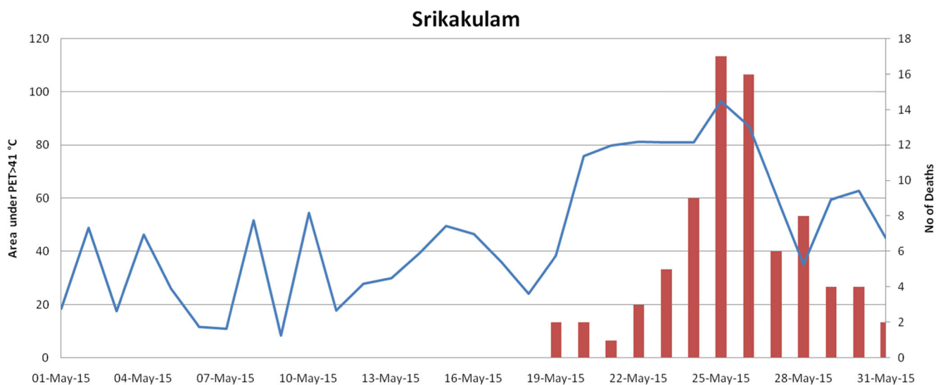
Fig. 10 Area under the curve (PET >41) and daily death rate at Srikakulam in May 2015
