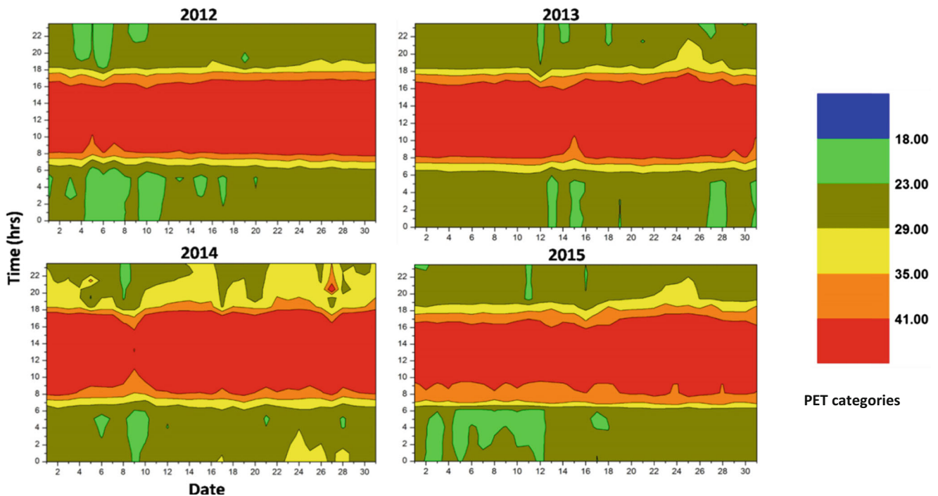
Fig. 6 PET (°C) over Srikakulam District of Andhra Pradesh during May
