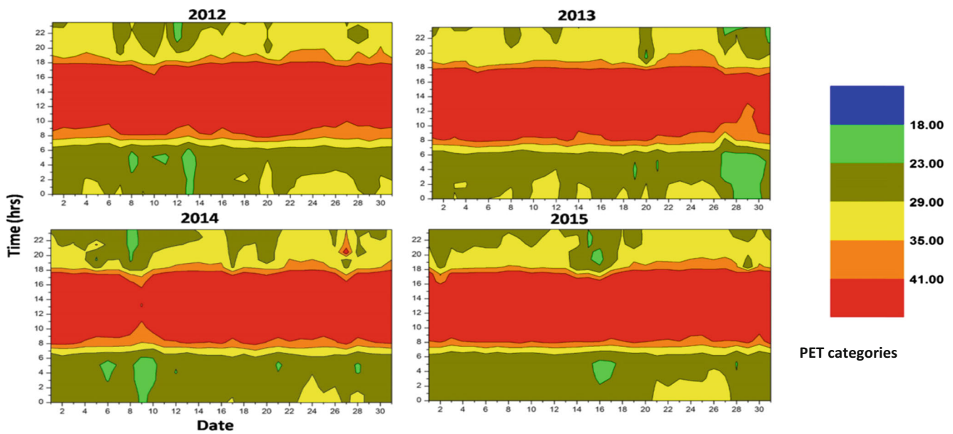
Fig. 5 PET (°C) over Kurnool District of Andhra Pradesh during May
